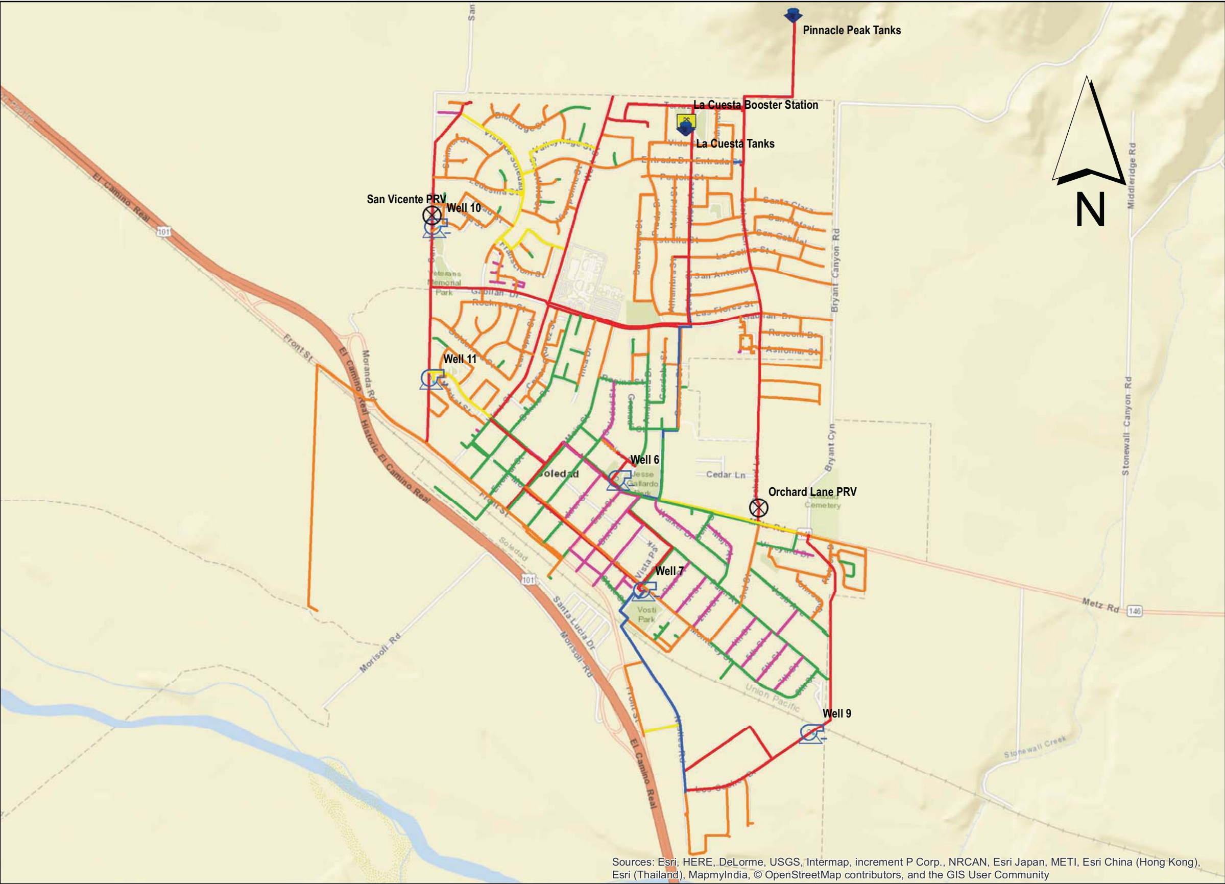
Figure 2.25 Map of Existing Pipes by Diameter
